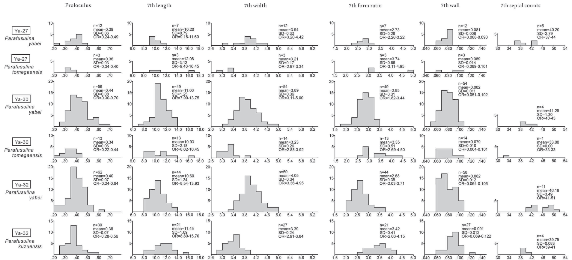
Figure 32. Frequency distribution histograms and statistical values [number of specimens (n), mean value, standard deviation (SD), and observed range (OR)] of diameter of six characters in Parafusulina yabei and P. tomegaensis from three samples of the lower part of the Nabeyama Formation. Numerical values in the vertical axis show the frequency and those in the horizontal axis in proloculus, 7th length, 7th width, and 7th wall (wall thickness of the seventh whorl) are shown in mm. These alphabetical symbols and numerical values in the vertical and horizontal axes are common in Figs. 32-35.
