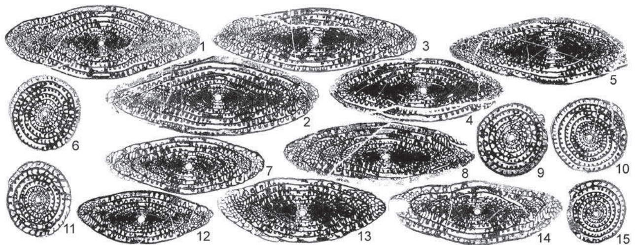
Figure 11. Parafusulina japonica in the Sample Ka-2. 6, 9-11, 15: sagittal sections; others: axial sections, all ×4.
