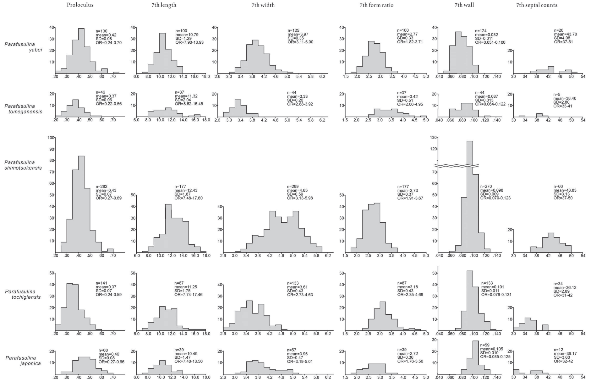
Figure 35. Frequency distribution histograms and statistical values in Parafusulina yabei , P. tomeganensis , P. shimotsukensis , P. tochiensis , and P. japonica in the Nabeyama Formation.
