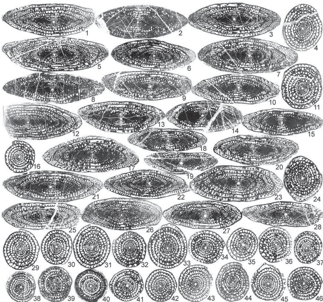
Figure 22. Parafusulina tochigiensis in the Sample Ka-70 (Part 2). 4, 11, 16, 24, 29-46: sagittal sections; others: axial sections, all \times 4 .
