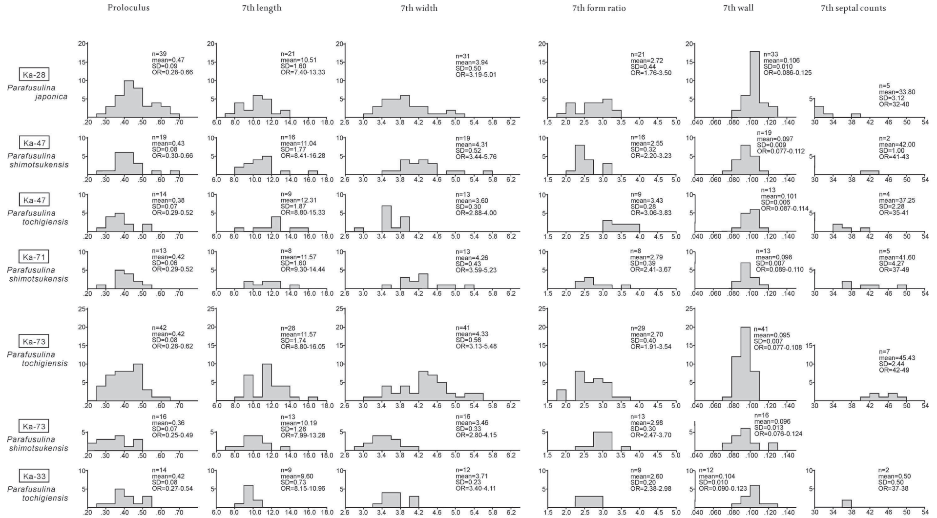
Figure 34. Frequency distribution histograms and statistical values in Parafusulina japonica , P. shimotsukensis , and P. tochiagensis from nine samples of the upper part of the Nabeyama Formation (Part 2).
