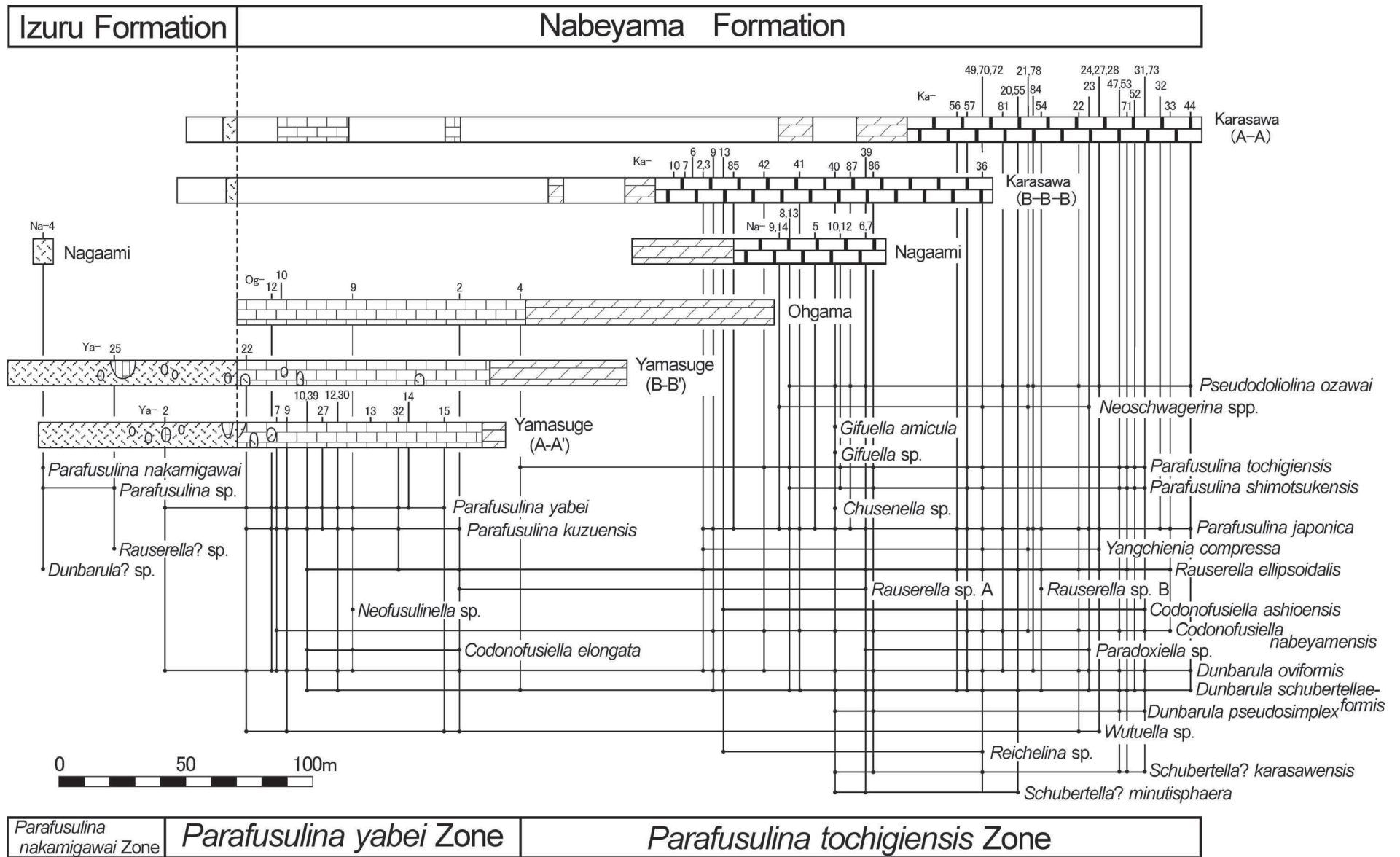
Figure 2. Stratigraphic distribution of fusulinoideans in the Izuru and Nabeyama formations, by which the Parafusulina nakamigawai , P. yabei , and P. tochigiensis zones were established from lower to upper (after Kobayashi, 2006b). For more geologic information see Kobayashi (2006a).
