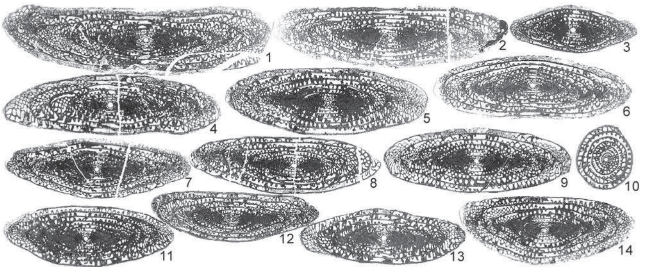
Figure 7. Parafusulina tomegansensis in the Sample Ya-30. 10: sagittal section; others: axial sections, all \times 4 .
